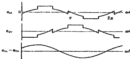
Fig. 5 Signal curve of three-phase PWM inverter by improving
