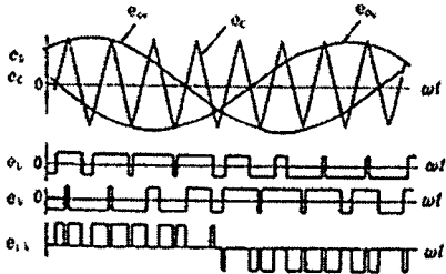
Fig. 4 Curve of three-phase PWM inverter
