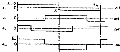
Fig. 3 PWM control by current estimation
