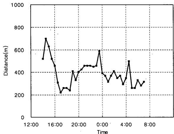
Fig. 9 Time-scale Distance between Ships of HANBADA's Ship-handling Result
