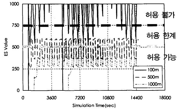
Fig. 7 Change Situation of Time Scale ES S Value
