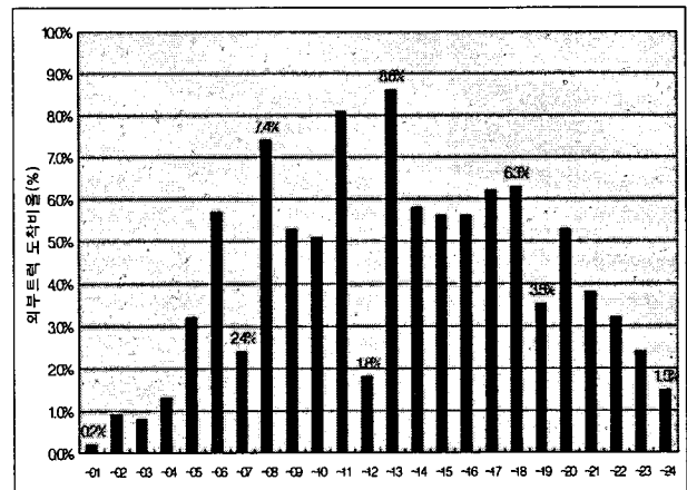
Fig. 1 Arrival distribution of gate-in
