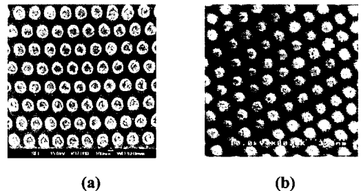
Fig. 3 SEM images of nano-pillar patterns with (a) 100 nm, and (b) 50 nm diameter on polymeric nano master by nano-UV imprint process (Polymeric nano-master, (a) and (b), was generated for electroforming process)
