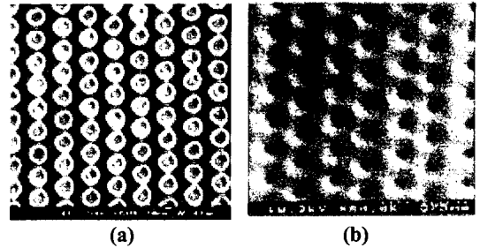
Fig. 2 SEM images of nano-hole patterns with (a) 100 nm and (b) 50 nm diameter on Si nano master by E-beam lithography and ICP etching
