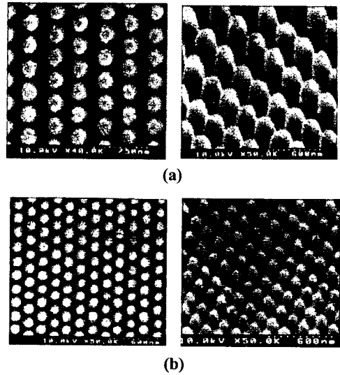
Fig. 6 SEM images of polymeric pillar patterns with (a) 100 nm, and (b) 50 nm diameter replicated by nano-injection molding process
