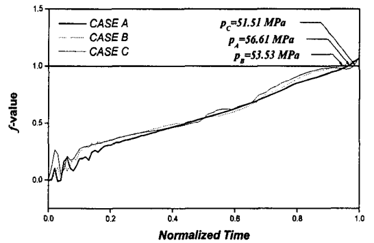
Fig. 3 Time histories of f -value for each load case
