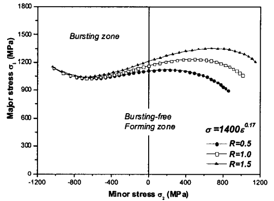
Fig. 1 Analytical forming limit stress diagram (FLSD)
