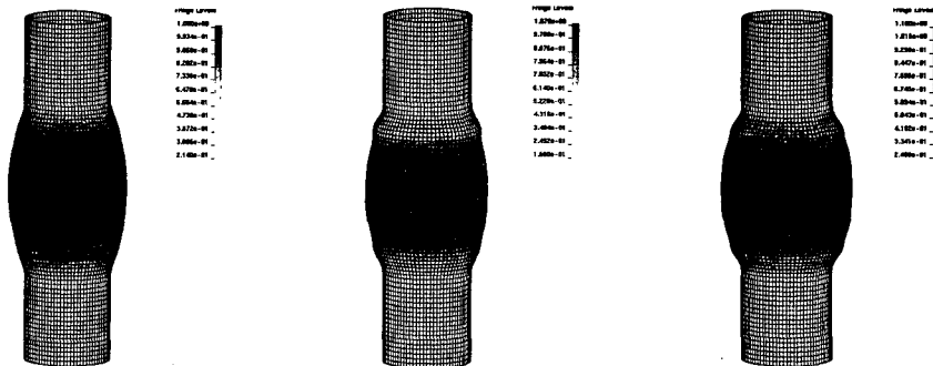
Fig. 4 Distributions of f -value at experimental bursting pressure value
