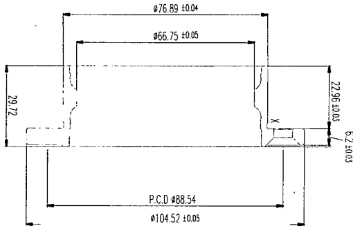
Fig. 1 A sectional diagram of the double angular ball bearing with flange.
