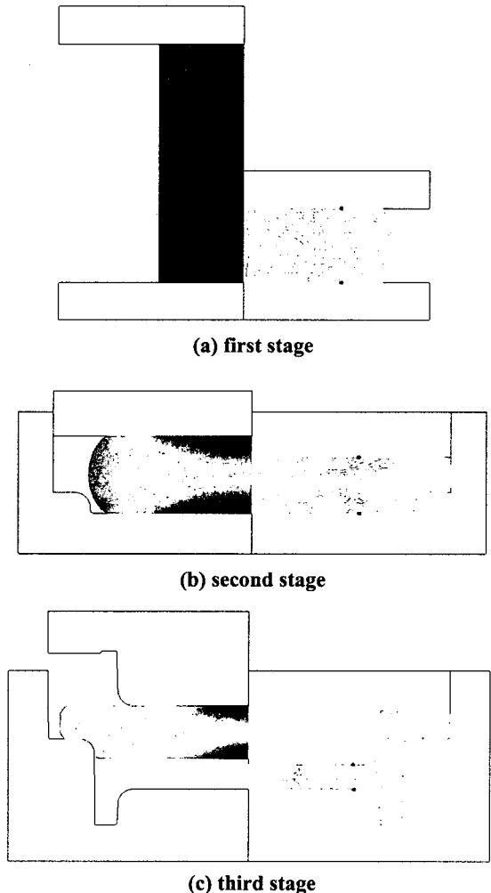
Fig. 2 Schematic description of a multi-stage hot forging process
