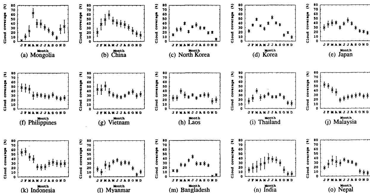
Figure 4: Country based statistics of monthly mean cloud coverage in Asia
