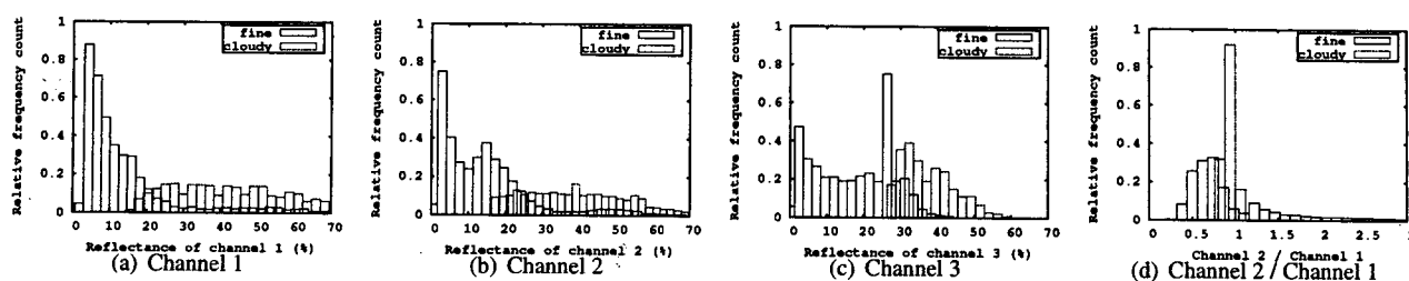
Figure 1: Histogram on AVHRR channel 1, 2 and 3 over fine and cloudy pixels.
