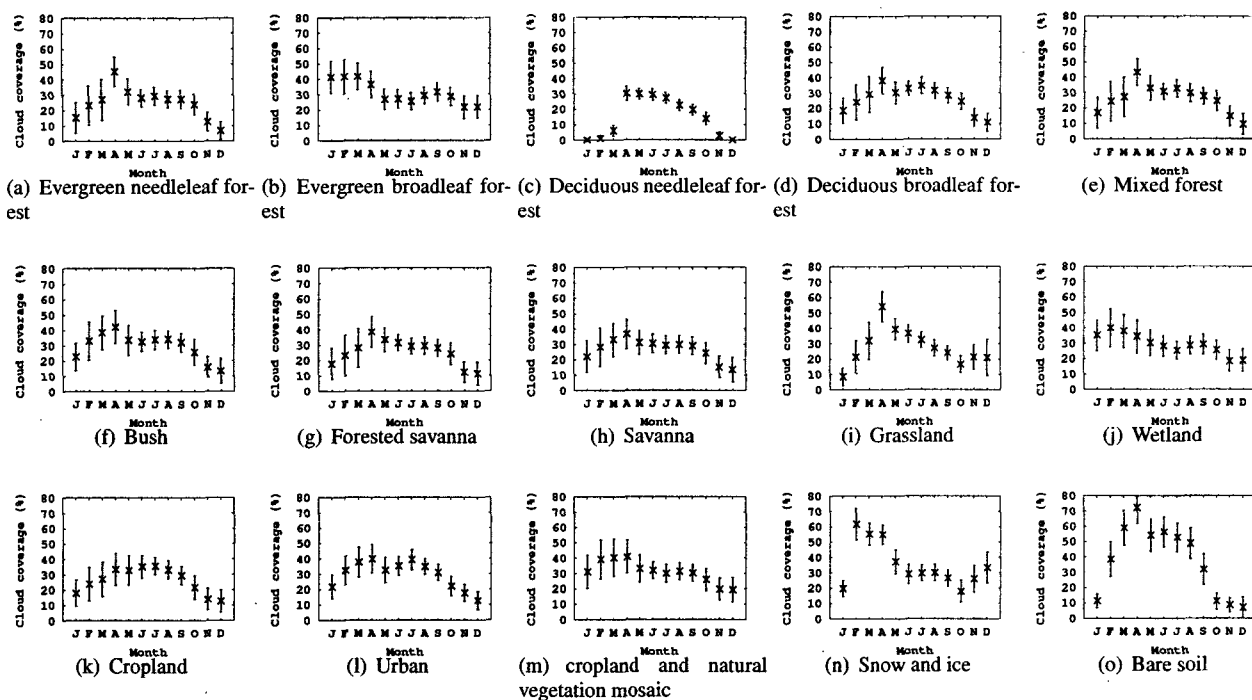
Figure 3: Land cover based statistics of monthly mean cloud coverage in Asia
