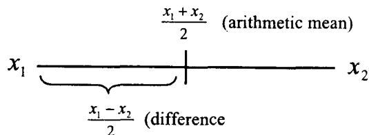
Figure 1. Basics of the Haar wavelet transform
