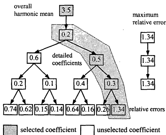
Figure 5. Greedy Algorithm
