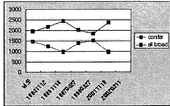
Figure 7. Changes of conifers and deciduous size
