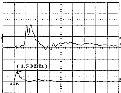
Ch.1 : discharge signal [ 1 V/div, 200 ns/div] Ch.A: FFT result [ 340 mV/div, 5 MHz/div]
