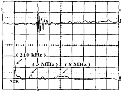
Ch.1 : discharge signal [ 10 mV/div, 500 ns/div] Ch.A : FFT result [ 0.91 mV/div, 5 MHz/div]
