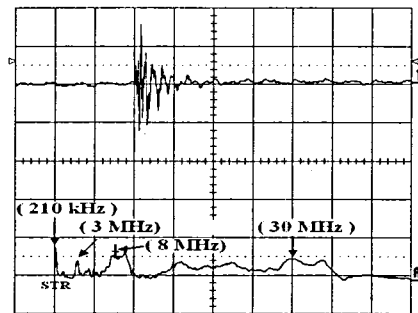
Ch.1 : discharge signal [20 mV/div, 500 ns/div] Ch.A: FFT result [ 0.91 mV/div, 5 MHz/div]
