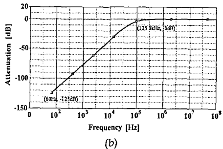
Fig. 3 Configuration(a) and frequency response(b) of the coupling network.
