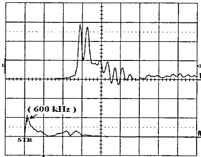
Ch.1 : discharge signal [ 1 V/div, 200 ns/div] Ch.A: FFT result [ 400 mV/div, 5 MHz/div]
