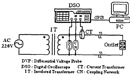
Fig. 2 Configuration of the experimental apparatus.
