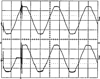
Ch.1 : voltage [200 V/div, 5 ms/div] Ch.2 : current [ 5 A/div, 5 ms/div]
