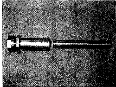
Fig. 6 Morphology of non-electric and delay explosive bolt after separation test.
