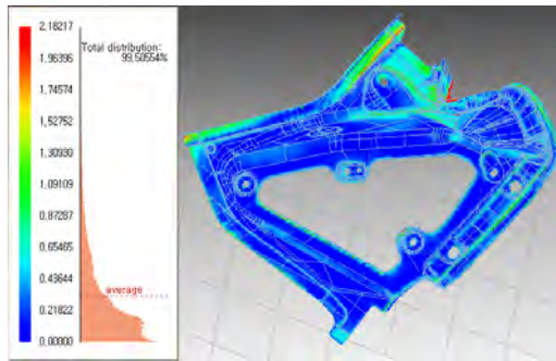
Fig. 7 Comparison of data between CAD and measurement
