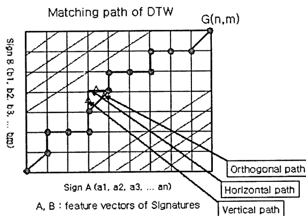
Fig. 3 Method of Dynamic Time Warping
