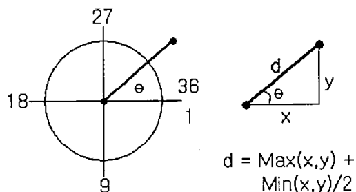
Fig. 2. Signature features of direction and distance
