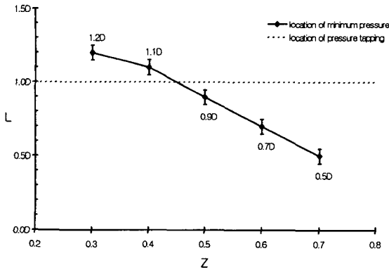
Fig. 5 Locations of the minimum static pressure at downstream of wedge element.
