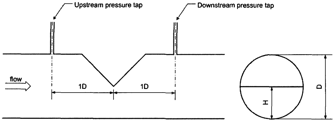
Fig. 2 Spool of segmental wedge
