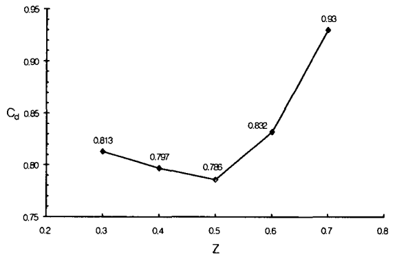
Fig. 4 Performance characteristics of discharge coefficients at various opening ratio.
