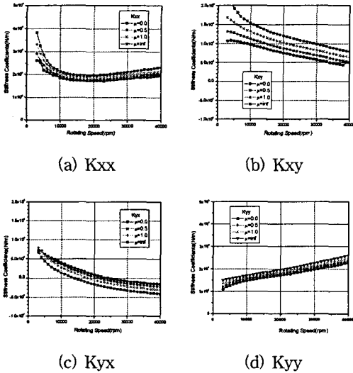
Fig. 9 Friction Effects on Stiffness Coefficients
