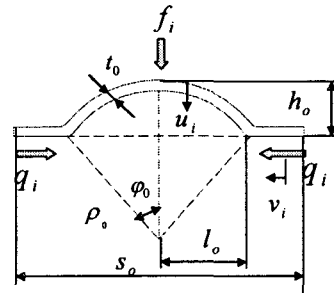
Fig. 2 Single Bump Configuration
