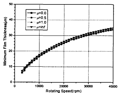
Fig. 8 Friction Effects on Minimum Film Thickness
