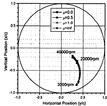
Fig. 7 Friction Effects on Rotor Locus
