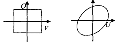
(a)Coulomb Damping (b)Viscous Damping
