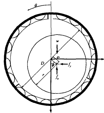
Fig.5 Coordinate system of AFB
