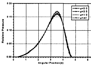
(a) Pressure distribution at \xi=1
