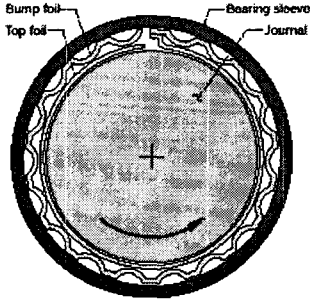
Fig.1 Bump type AFB
