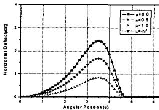
(c) Horizontal deflection distribution at \xi=1
