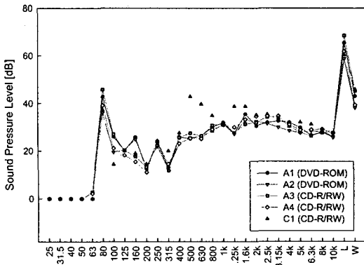
(a) 5000 rpm
