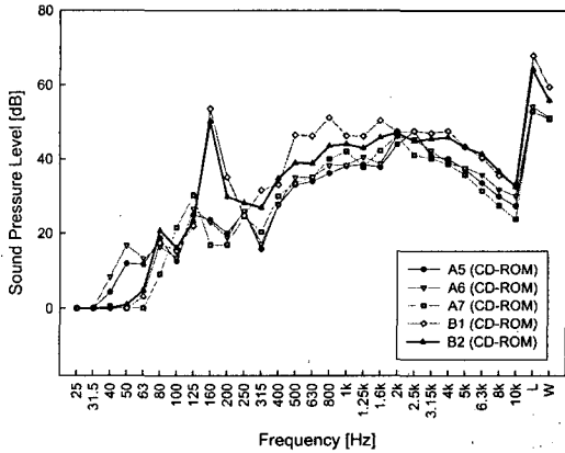
Fig. 6 Comparison of sound pressure level at maximum operation speed for different CD-ROMs
