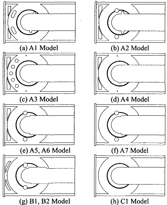
Fig. 5 Geometric planform configurations of several tray models used in the present experimental tests.
