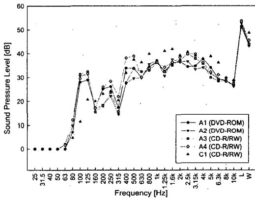
(b) 6800 rpm
