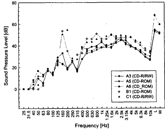
Fig. 8 Comparison of sound pressure level in 52X ODD
