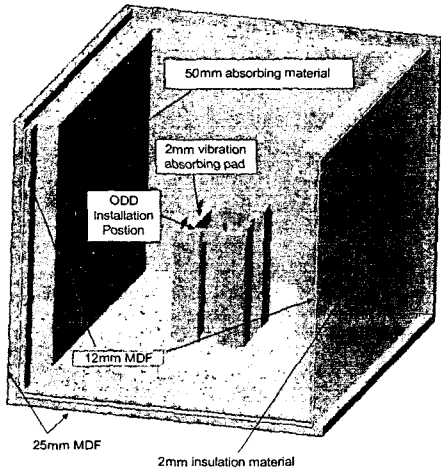
Fig. 1 Conceptual diagram of the sound insulation case
