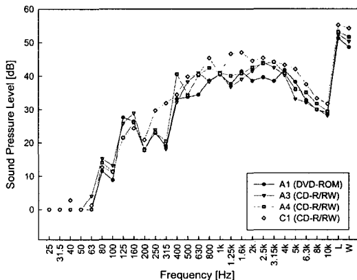
(c) 8600 rpm
