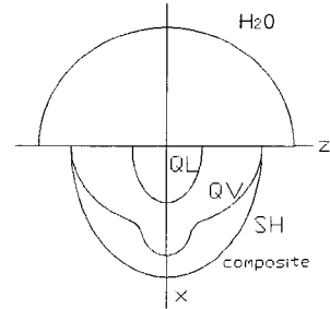
Fig. 4 The slowness surface (parallel to fiber)
