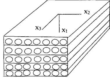
Fig. 2 Coordinate system in unidirectional reinforced composites
