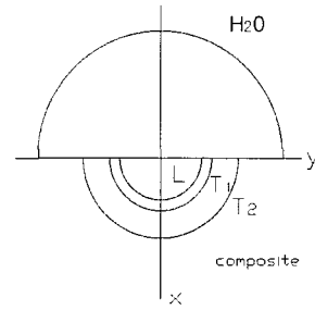
Fig. 3 The slowness surface (transversely isotropic plane)
