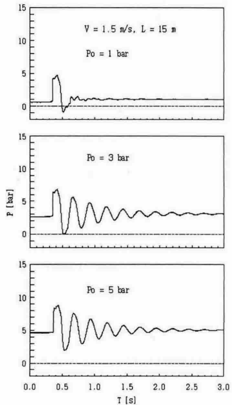
Fig. 5 Effect of flow velocity on pressure histories(L=15 m, V=1.5 m/s).
