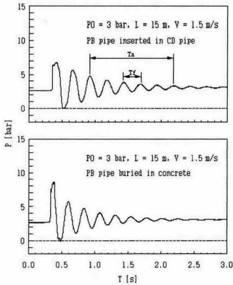
Fig. 2 Effect of polybutylene pipe inserted in CD pipe and buried in concrete on pressure histories ( L=15 m, P_o=3 bar).
