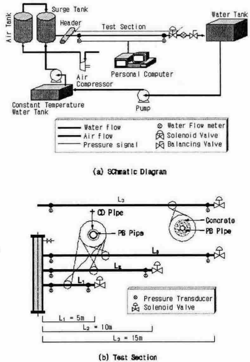
Fig. 1 Schematic diagram of the experimental apparatus.
