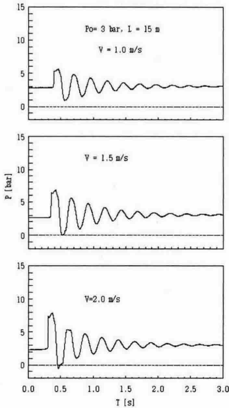
Fig. 4 Effect of flow velocity on pressure histories(L=15 m, Po=3 bar).
