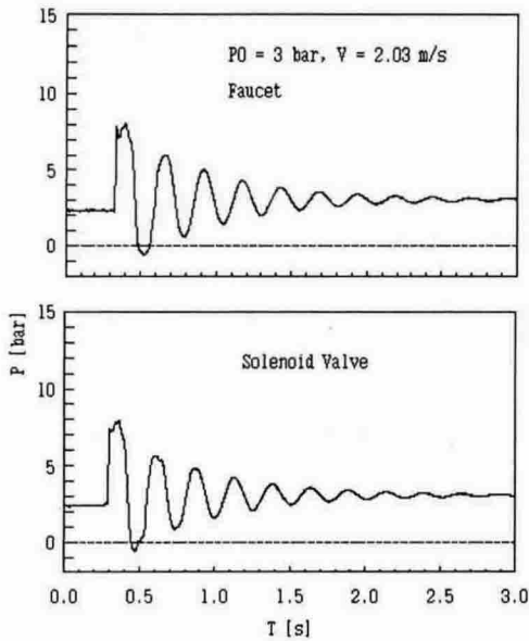
Fig. 6 Effect of faucet and solenoid valve on pressure histories (L = 15 m, Po = 3 bar, V = 2.03 m/s).
