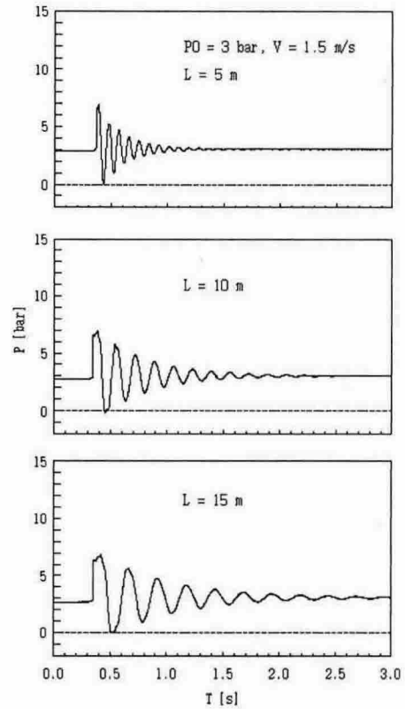
Fig. 3 Effect of pipe length l on pressure histories ( P_o=3 bar, V=1.5 m/s).
