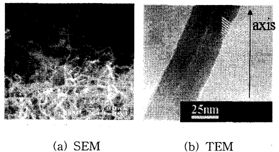
Fig. 1. CNF structure of (a) SEM and (b) TEM image
