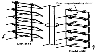
Fig. 1 Principle of opening-shutting door
