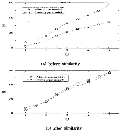
Fig. 12 Distribution of revolution with wind velocity for miniature and prototype model
