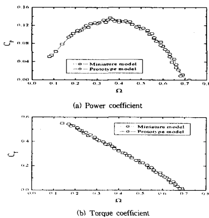
Fig. 13 Comparison of tip speed ratio versus power and torque coefficient for prototype and miniature model
