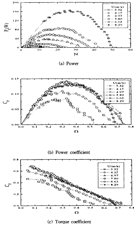
Fig. 11 Distribution of P_r , C_r , C_t and tip speed ratio for variation of wind speed at prototype model turbine
