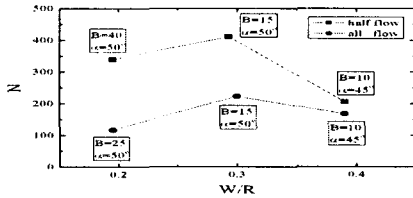
Fig. 7 Distribution of maximum revolution with angle, number and aspect ratio of blade
