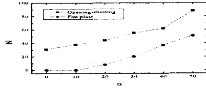
Fig. 9 Comparison of revolution with flat plate and opening-shutting blade
