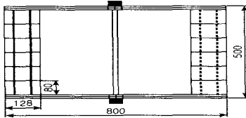
Fig. 4 Schematic diagram of miniature wind turbine using opening-shutting door
