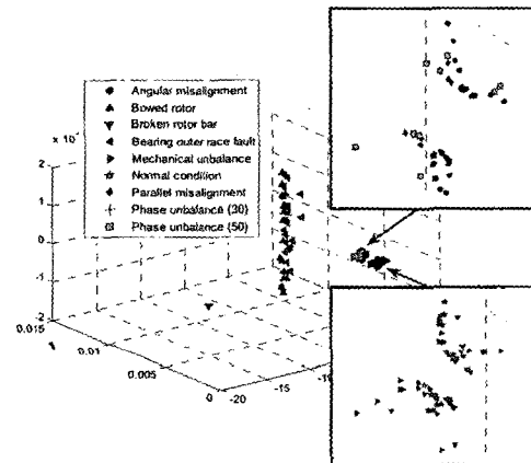
Fig. 3 The feature of motor faults
