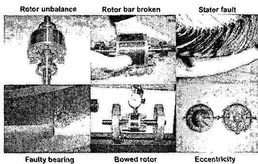
Fig. 2 Fault images of induction motors
