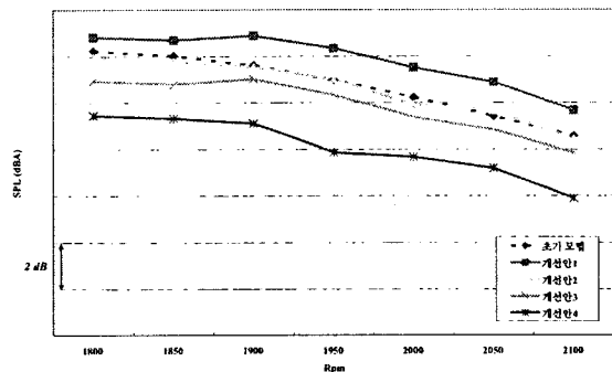
Fig. 10 Noise level in the engine room after the modification of tail-pipe
