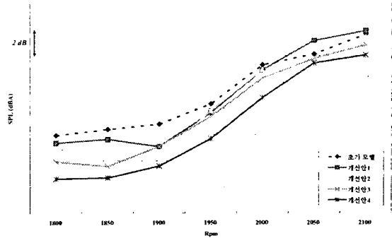
Fig. 9 Cabin noise level after the modification of tail-pipe
