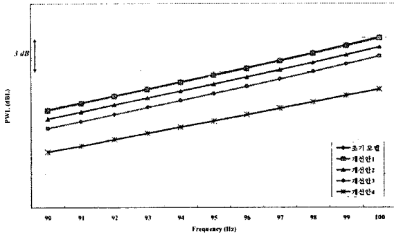
Fig. 8 Noise analysis result for modified tail-pipe
