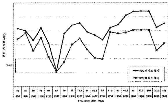
Fig. 3 Cabin noise level without/with tail-pipe
