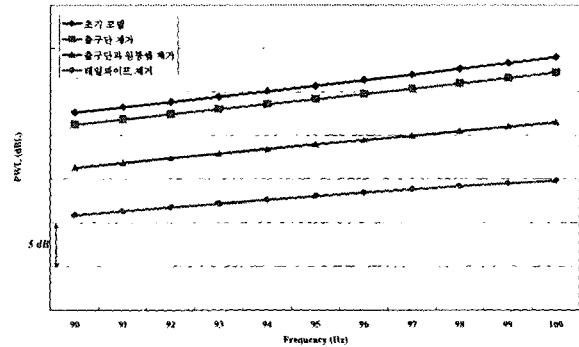
Fig. 7 Noise contribution due to each part of tail-pipe
