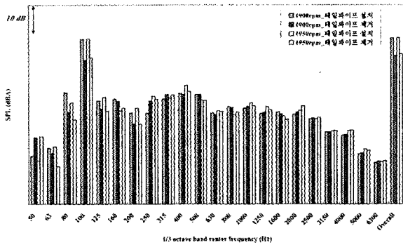
Fig. 2 Cabin noise level at main operating rpm
