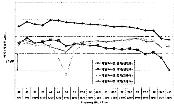
Fig. 4 Noise level at the tail-pipe and engine room without/with tail-pipe
