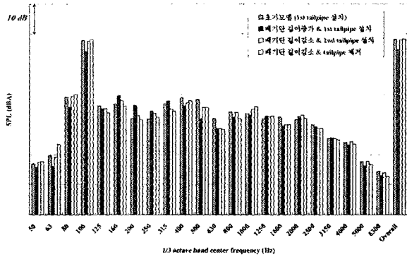
Fig. 5 Cabin noise level according to the various tail-pipes and exhaust tubes
