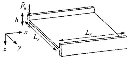
Fig. 3. A coupled structure consisting of two finite beams attached to a rectangular plate.
