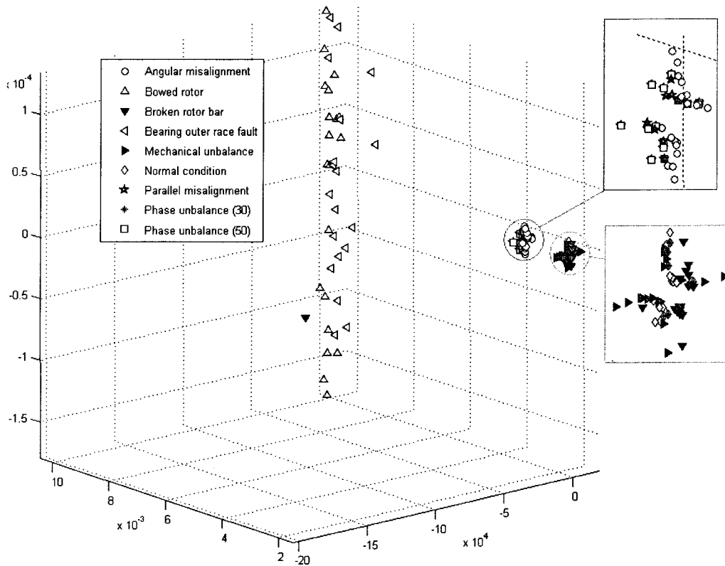
Fig. 3 The feature of motor faults
