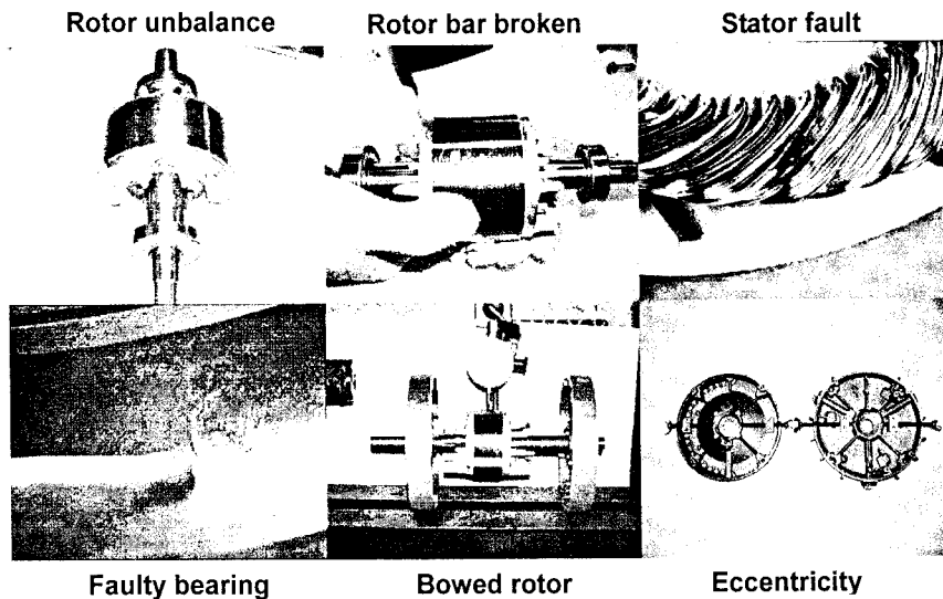
Fig. 2 Fault images of induction motors
