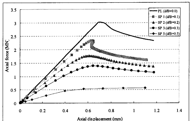
Fig. 3 Relationship between axial force and displacement
