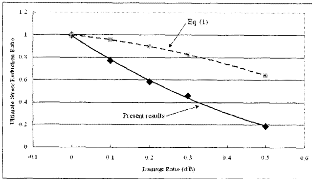
Fig. 4 Variation of the ultimate strength of damaged stiffened plates
