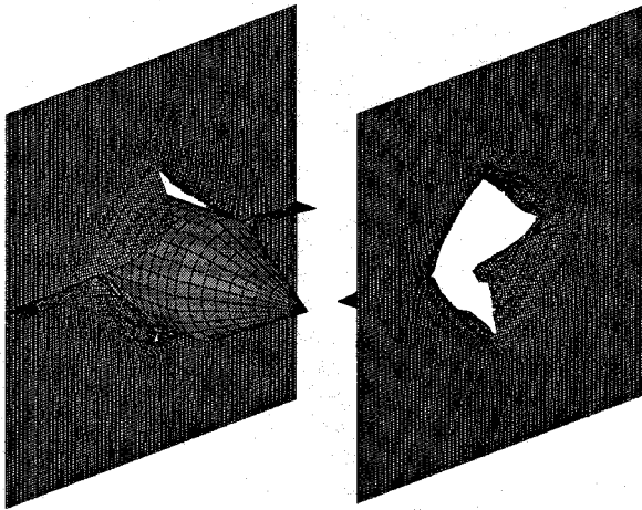
Fig. 2 Generated minor collision damage ( d/B=0.3 )
