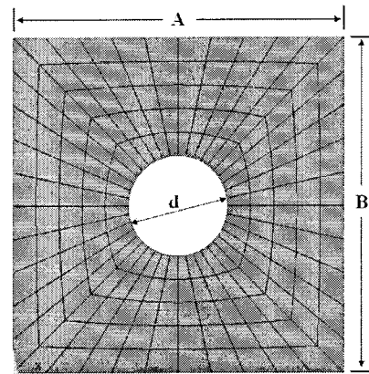
Fig. 1 Typical mesh of a perforated plate
