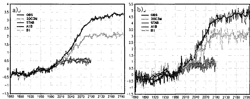
Fig. 2. Time series of surface temperature anomalies from 1860 to 2200: a) global mean, and b) East Asia mean (Observation (1860-2000), 20C3M (1860-2000), STAB (2001-2100), A1B (2001-2200), and B1 (2001-2200) simulations are shown).
