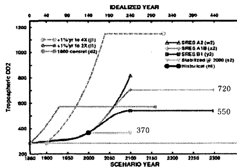
Fig. 1. CO2 concentration (ppm) in AR4 experiment.
