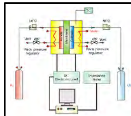
Fig. 1 Schematic diagram of the unit cell performance test station.
