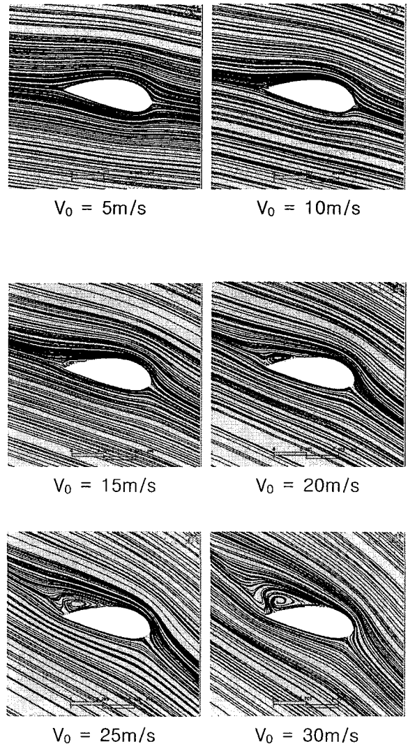
Fig. 2 The streamlines around moving blade
