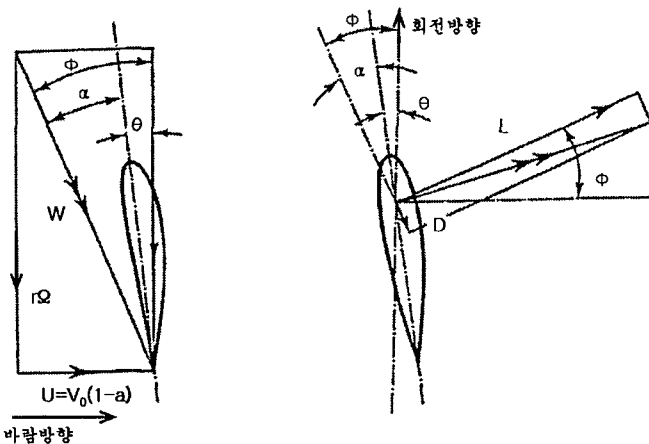
Fig. 1 Relative flow velocities
