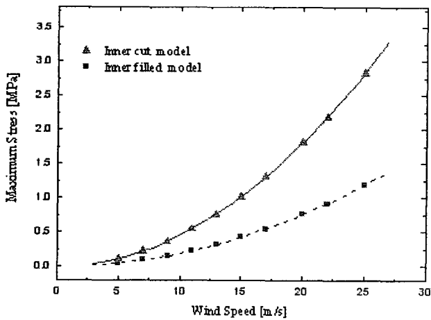
Fig. 5 Maximum Stress
