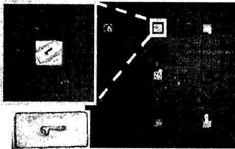
Photo. 2. Digital microscope image of sensor array. The particles arranged on the chip by magnetic force interaction.
