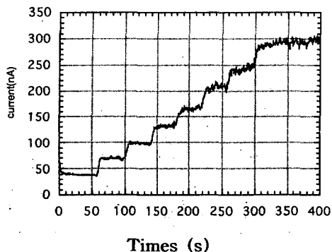
Fig. 2. Electrochemical response curve of the electrode on the chip against the sequential addition of hydrogen peroxide.
