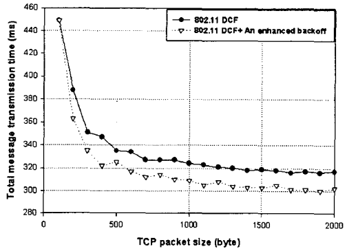
Fig. 2 Total message transmission time ( E_b/N_0 = 4 dB)
