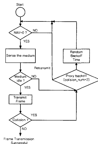
Fig. 1 Flowchart of Proposed IEEE 802.11 MAC protocol
