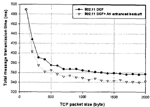
Fig. 3 Total message transmission time ( E_b/N_0 = 4 dB, K_R = 9 dB, Rician)
