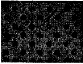
Fig.7 microscopy of diffraction grating (a) dot pitch 4um, (b) dot pitch 4um ,10um (c)dot pitch 10um
