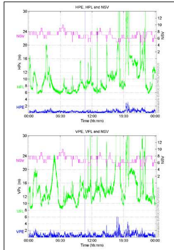
Figure 11. SBAS Position Error, Protection Levels and NSV used in position solution.
