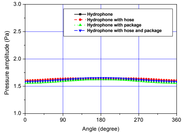
Fig. 7 Pressure distribution around hydrophone with respect to the angle at 3kHz
