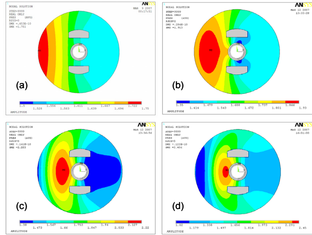
Fig. 5 Pressure distribution of hydrophone and package at; (a) 3kHz, (b) 6kHz, (c) 9kHz, and (d) 12kHz.
