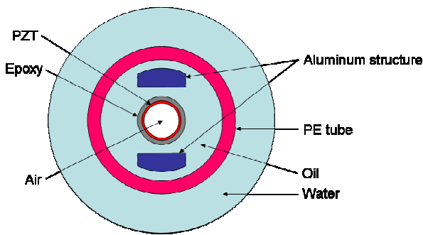
Fig. 1 Schematic diagram of hydrophone system.
