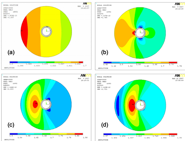
Fig. 3 Pressure distribution of single hydrophone at; (a) 3kHz, (b) 6kHz, (c) 9kHz, and (d) 12kHz.
