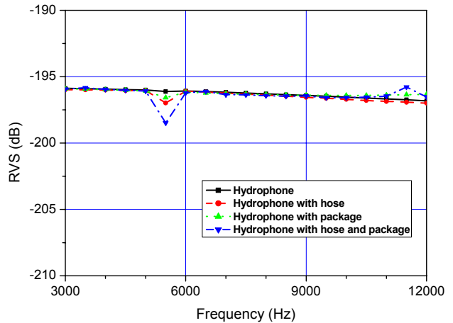
Fig. 11 Receiving voltage response(RVS) of hydrophone
