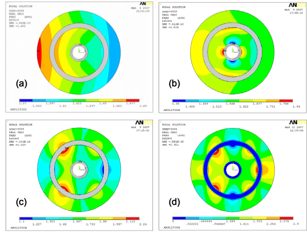
Fig. 4 Pressure distribution of hydrophone and hose at; (a) 3kHz, (b) 6kHz, (c) 9kHz, and (d) 12kHz.
