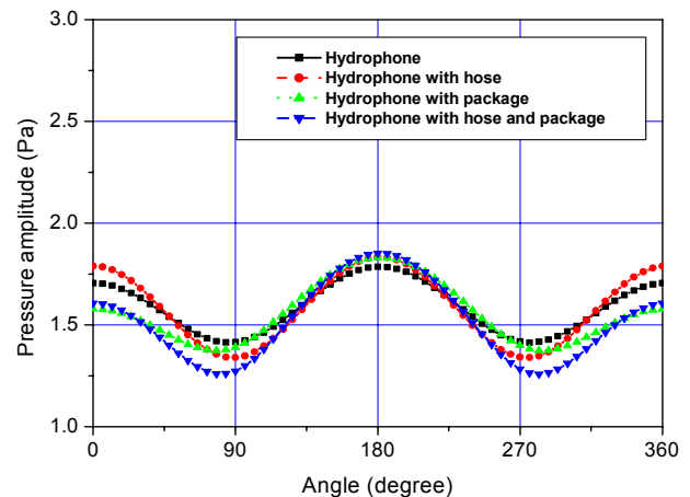
Fig. 8 Pressure distribution around hydrophone with respect to the angle at 6kHz
