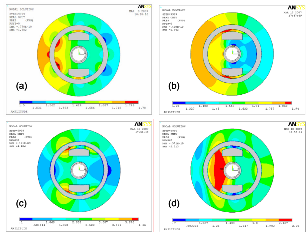
Fig. 6 Pressure distribution of hydrophone system at; (a) 3kHz, (b) 6kHz, (c) 9kHz, and (d) 12kHz.
