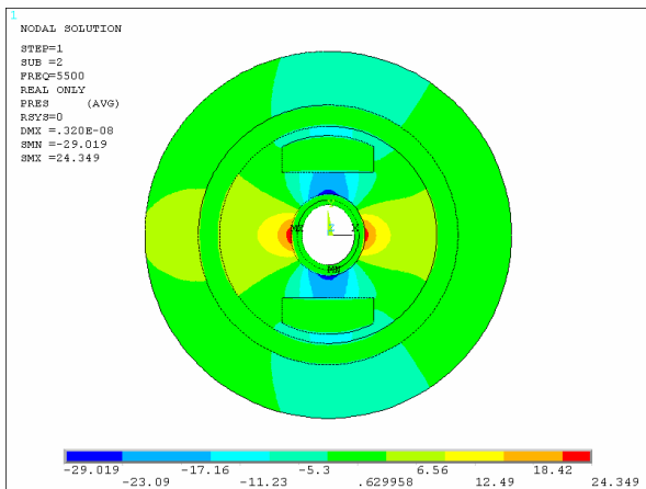
Fig. 12 Pressure distribution of hydrophone system at 5.5kHz
