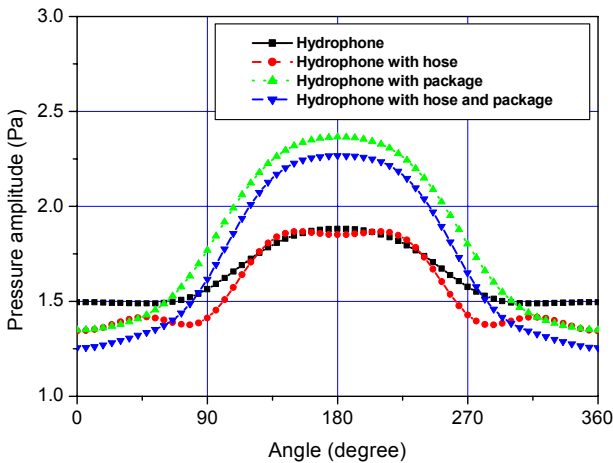
Fig. 10 Pressure distribution around hydrophone with respect to the angle at 12kHz
