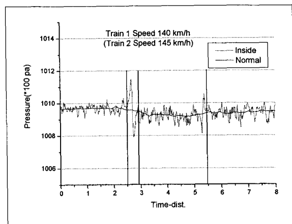
Fig. 9. Pressure Variation(Velocity 285km/h)
