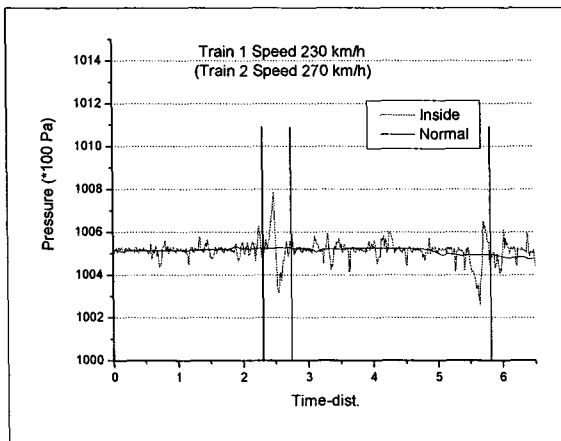
Fig. 6. Pressure Variation(Velocity 500km/h)
