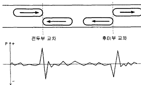
Fig 5. Pressure Variation Pattern of Passing Trains
