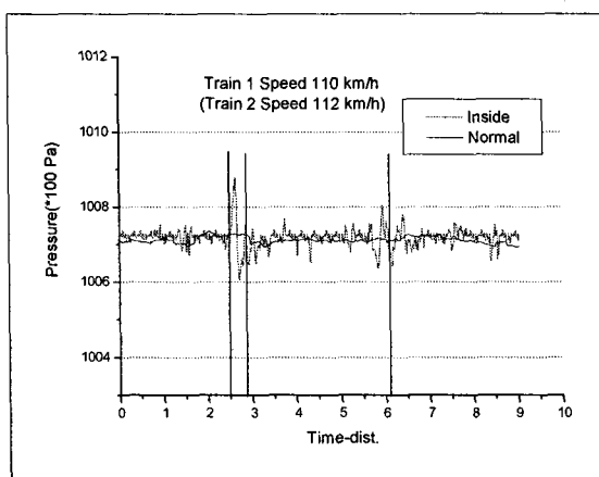
Fig. 8. Pressure Variation(Velocity 222km/h)
