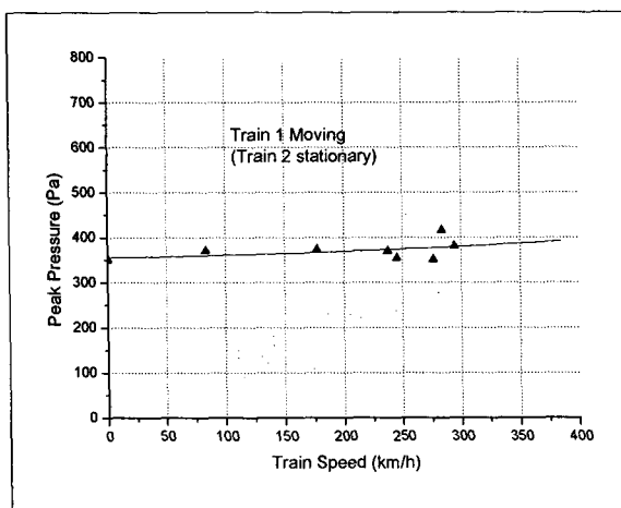
Fig. 10. Pressure Variation(Train 2 Stop)
