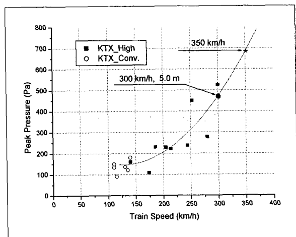
Fig. 11. Peak Pressure to Train Speed
