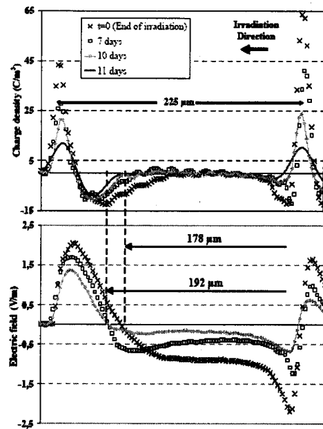
Fig. 1. Kapton sample 225 m-thick charge density recorded by PEA and electric field calculated during the relaxation after 30 mn irradiation under 150 keV with a flux of 125 pA/cm 2 .
