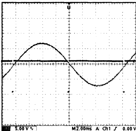
(a) R_L = 100K\Omega
