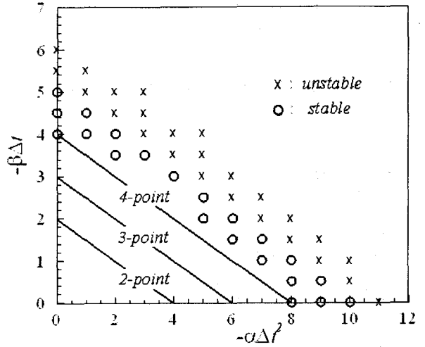
Fig. 4 Stability regimes in 2-D flow
