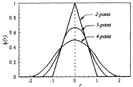
Fig. 2 Three types of regularized delta functions
