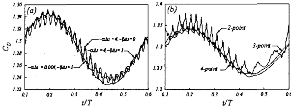
Fig. 8 Time history of the drag coefficient (a) for different forcing gain using 3-point delta function (b) for different types of delta functions with -\alpha\Delta t^2 = 0.4, -\beta\Delta t = 1
