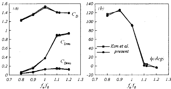
Fig. 9 Variations of the force coefficients and phase angle with respect to f_c/f_0 (a) mean drag coefficient and rms drag and lift fluctuation coefficients (b) phase angle between C_L and the vertical position of the cylinder.
