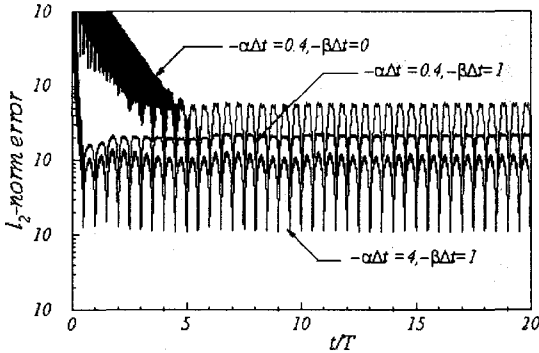
Fig. 7 l_2 - norm error of the virtual surface velocity in the stream-wise direction normalized by the free-stream velocity u_\infty for three different forcing gains
