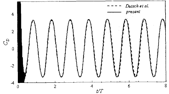
Fig. 6 Time history of the drag coefficient
