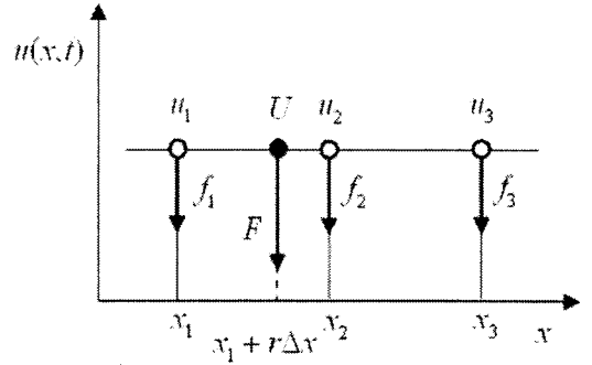
Fig. 3 Virtual boundary velocity and forcing in 1-D space
