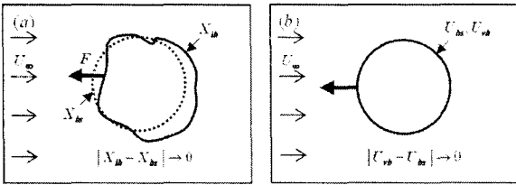
Fig. 5 Schematic diagram for comparison of two method (a) Peskin's IB method (b) virtual boundary method
