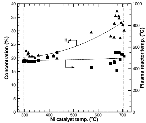
Fig. 6. The effect of catalyst reaction temperatures.
