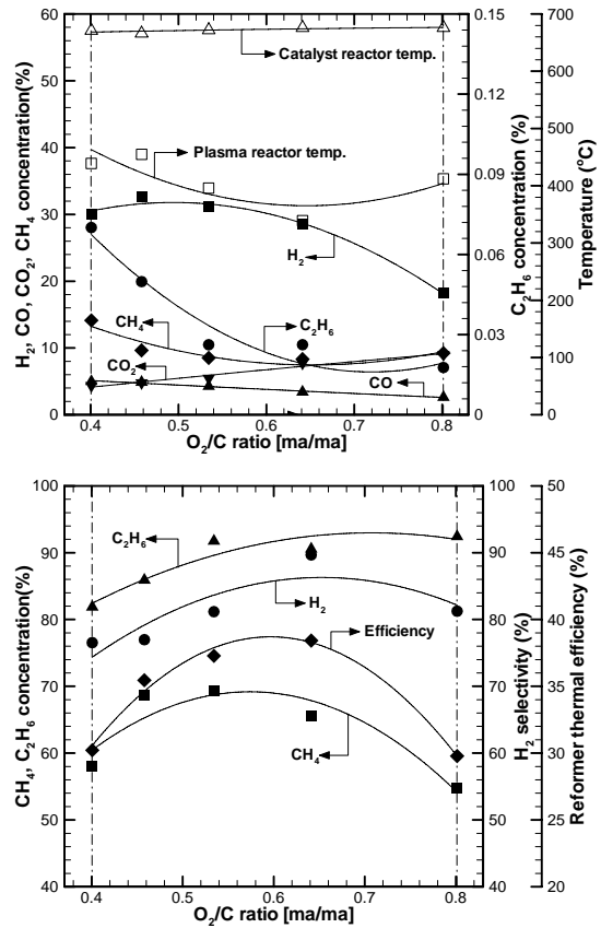
Fig. 4 The effect of the various O 2 /C ratios.
