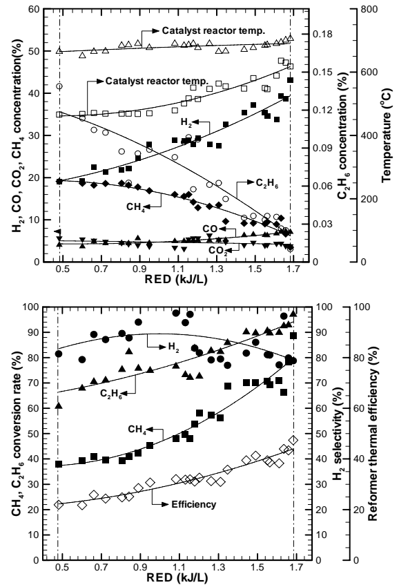
Fig. 7 The effect of the various input power levels.
