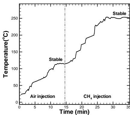
Fig. 2 Initial operating characteristics of the GlidArc plasma reformer.
