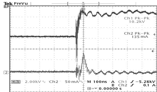
Fig. 3 Voltage and current characteristics of the GlidArc plasma reformer.
