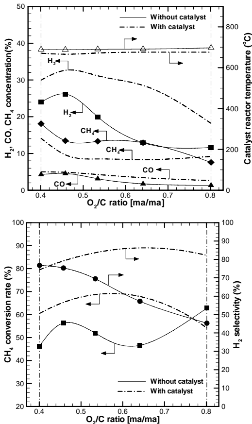
Fig. 8 The effect of the case with and without a catalyst.
