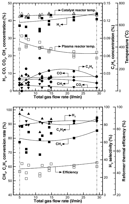
Fig. 5 The effect of the various flow rates.
