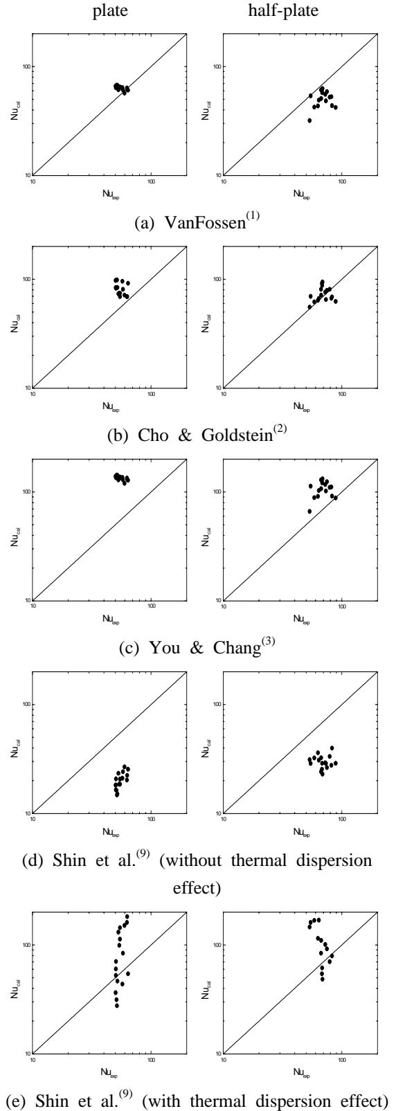
Fig. 3 Comparison of the Nu_{exp} and Nu_{cal}
