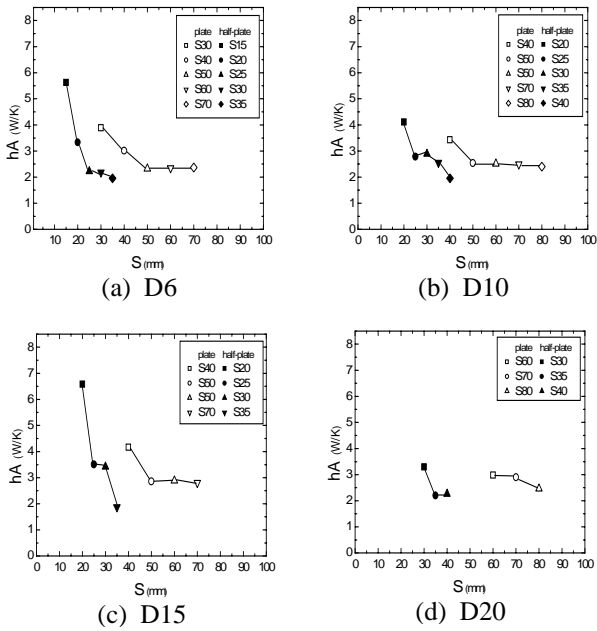
Fig. 4 Variation of the product of heat transfer coefficient and area with pitch (experiment).
