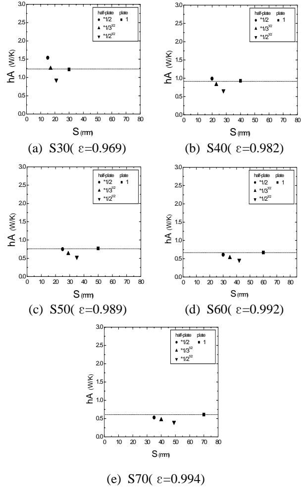
Fig. 5 Variation of the product of heat transfer coefficient and area with pitch (calculation).
