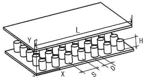
Fig. 2 Sketch of a channel with pin-fin array.
