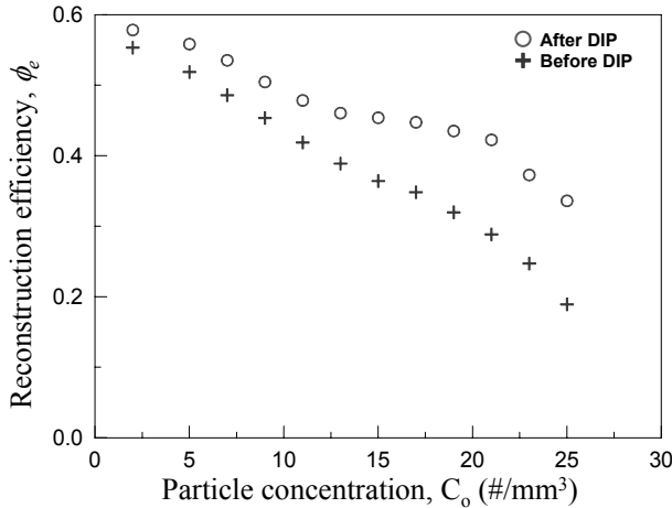
Fig. 4 Comparison of reconstruction efficiency with and without digital image processing procedure
