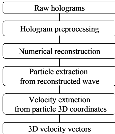
Fig. 2 Flowchart of digital in-line HPTV technique
