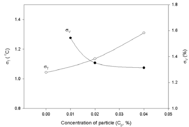
Fig. 7 Variation of temperature error \sigma_T and velocity error \sigma_v with respect to concentration of particle.
