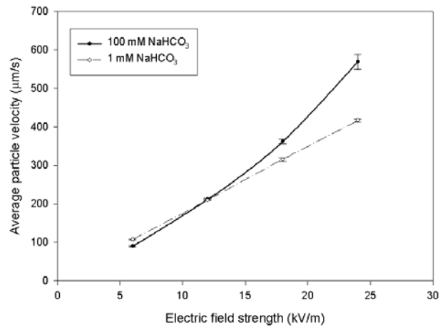
Fig. 10 Averaged apparent particle velocity with respect to electric field strength.
