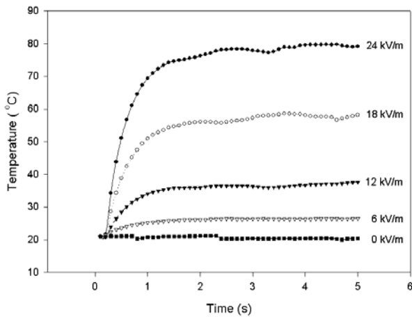
Fig. 8 Mean temperature variation with respect to time and electric field strength.
