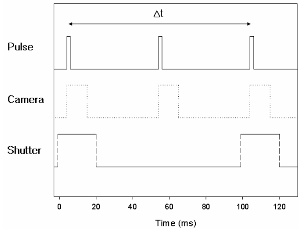
Fig. 1 Timing diagram.
