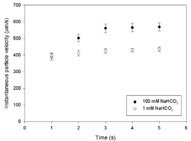
Fig. 11 Instantaneous apparent particle velocity at 24 kV/m.
