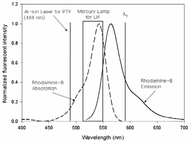
Fig. 3 Spectra characteristics of rhodamine-B and optical system.
