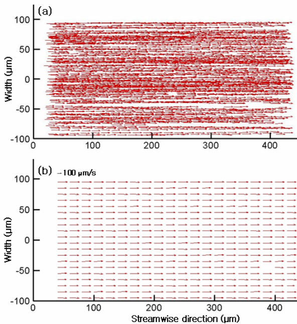
Fig. 9 PTV results at 12 kV/m: (a) total velocity vectors from 650 PTV images, (b) spatially averaged velocity field.
