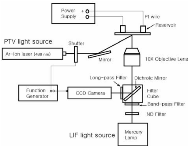
Fig. 4 Schematic of experimental apparatus for simultaneous measurement system.
