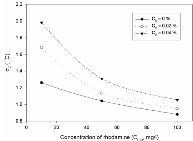
Fig. 6 Variation of temperature error \sigma_T with respect to concentration of rhodamine-B and particle.
