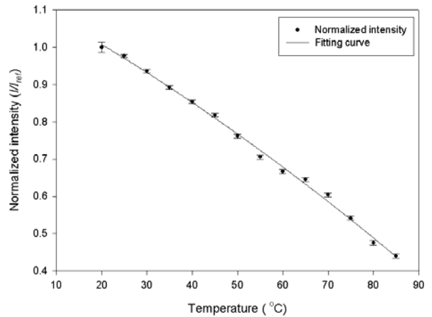
Fig. 5 Normalized calibration data and second-order polynomial fitting curve.
