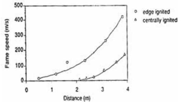
Fig. 4 Flame speed vs. distance for centrally and edge ignited explosions in a double configuration(i.e. solid top plate) with obstacles
