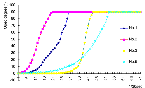
Fig. 6 Open degree of Vent port
