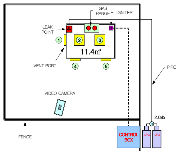
Fig. 2 Experimental apparatus
