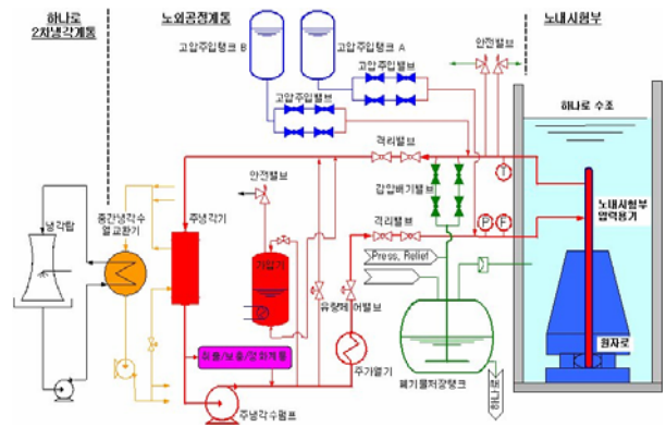
Fig. 1 Schematic Diagram of FTL
