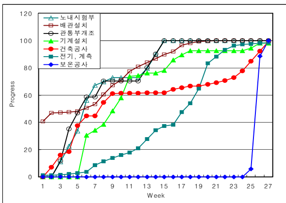
Fig. 8 Construction Progress of the Parts
