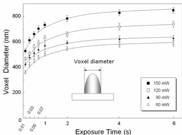
Fig. 3 Variation of voxel diameter according to laser power and exposure time.
