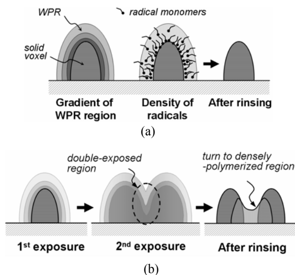
Fig. 4 (a) Schematic illustration of radical density around a fully polymerized voxel and (b) mechanism of the generation of thin pattern having sub-30 nm between voxels by overlapping WPRs.
