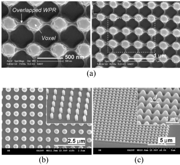
Fig. 5 SEM images of fabricated patterns: (a) embossing patterns having thin lines between voxels fabricated under laser power of 60 mW and exposure time of 30 ms per voxel; (b) perfect dot patterns and (c) merged dot-patterns generated by different voxel distance, d .
