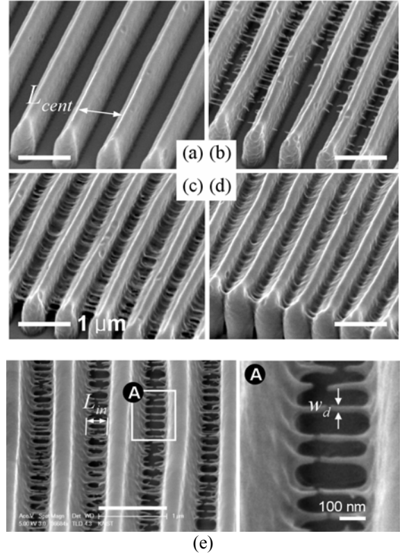
Fig. 6 SEM images of fabricated nanofibers with varying central distance ( L_{cent} ): (a) 900 nm, (b) 770 nm, (c) 670 nm, and (d) 620 nm, respectively. The scale bars are 1 \mu m. (e) Well-fabricated nanofibers among the densely-polymerized line patterns. The distance between lines ( L_{in} ) was approximately 270 nm, and the diameters ( W_d ) of the nanofibers are 20 to 30 nm.
