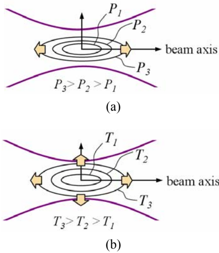
Fig. 1 Schematic diagram of (a) 'P-scheme' for voxel formation ( P : laser power) and (b) 'T-scheme' for voxel growth ( T : laser exposure time).
