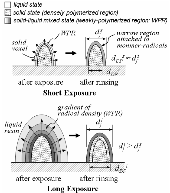
Fig. 2 Schematic illustration of voxel generation between short-exposure and long-exposure. Three different regions exist: fully (densely)-polymerized region, weakly-polymerized region, and liquid state.
