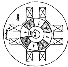
Fig. 1. Cross section of the generator.
