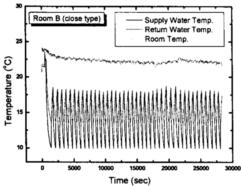
Fig. 6 Indoor air temperature and load side water temperature variation of close type heat pumps
