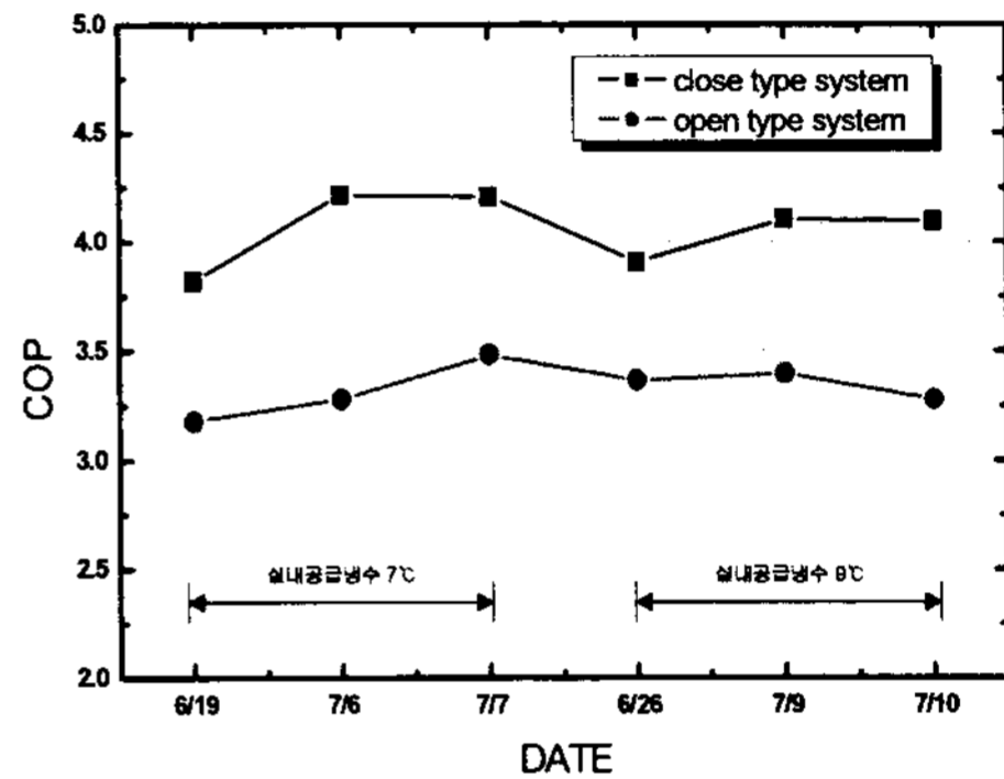
Fig. 9 Heat pump system COP in cooling mode with load side circulating water temp
