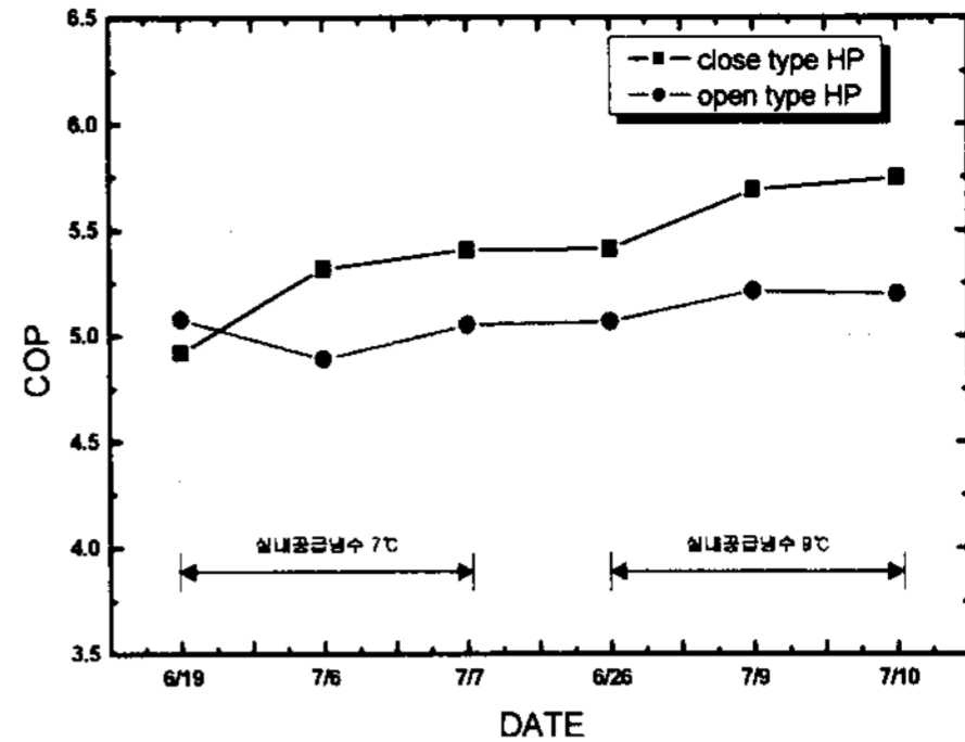
Fig. 8 Heat pump COP in cooling mode with load side circulating water temp
