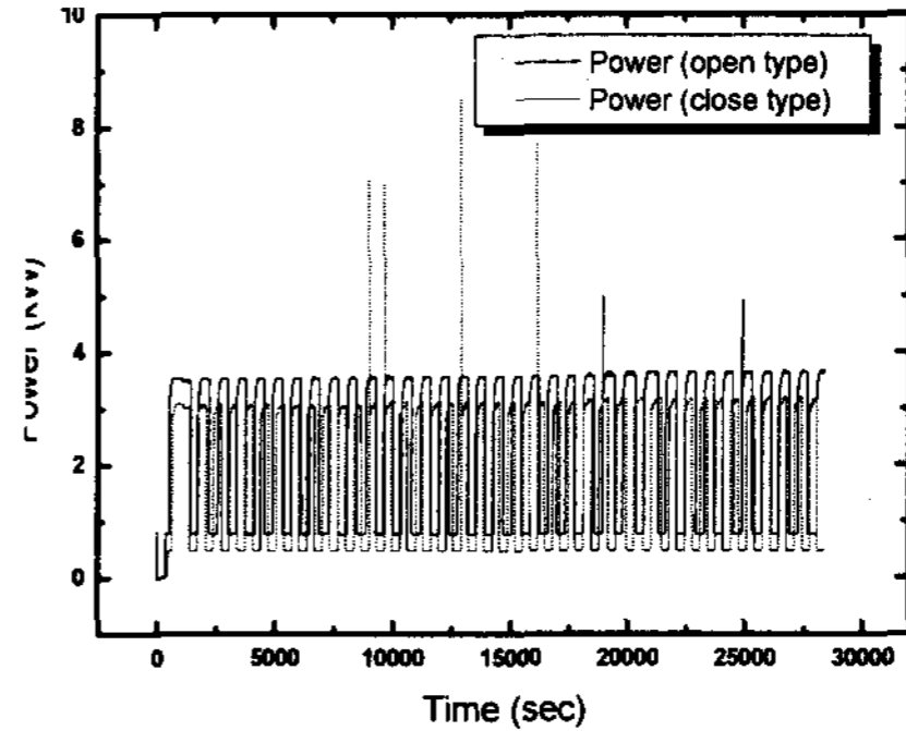
Fig. 2 Power consumption of heat pumps
