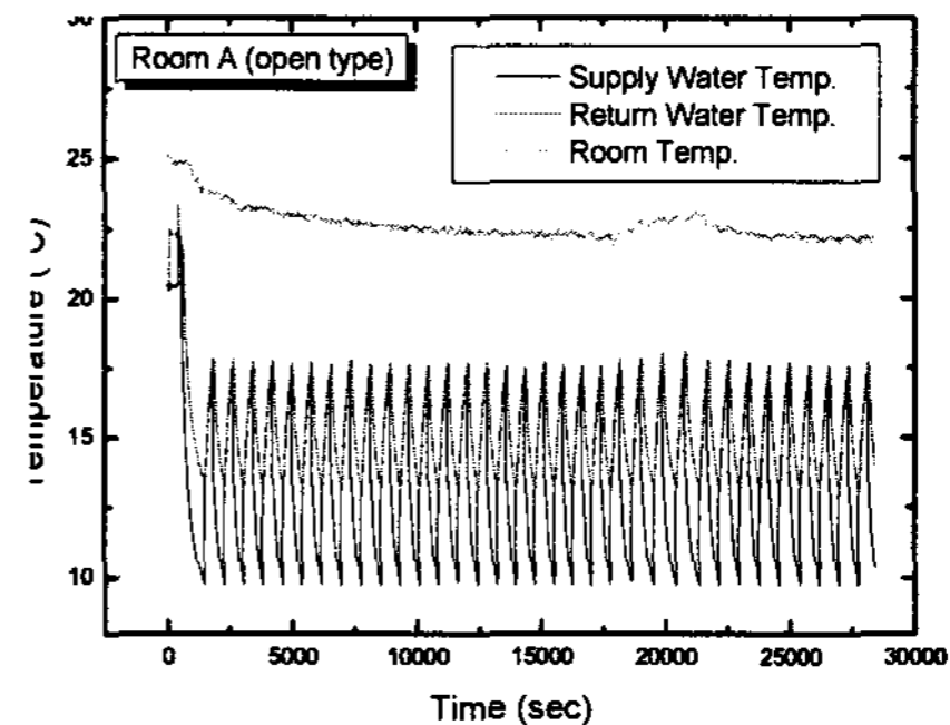
Fig. 4 Indoor air temperature and load side water temperature variation of open type heat pumps
