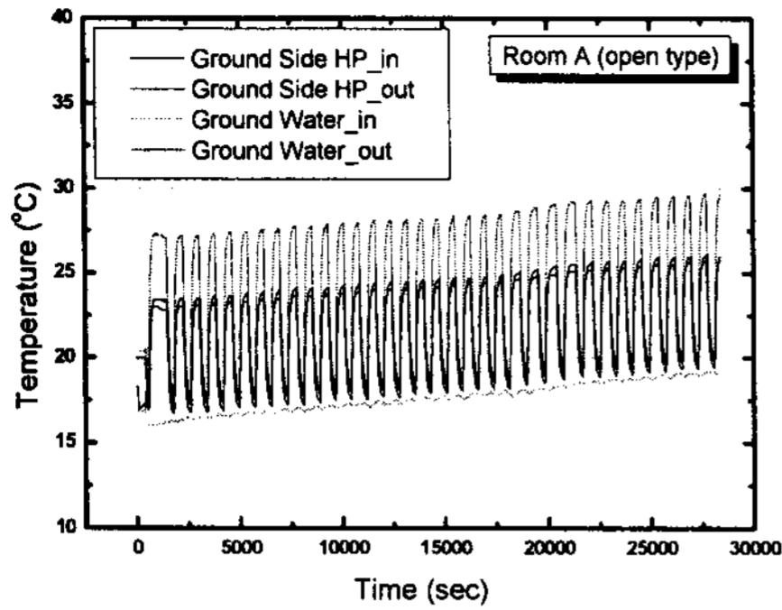
Fig. 5 Ground side water temperature variation of open type heat pumps
