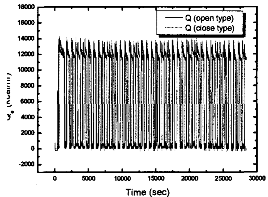
Fig. 3 Cooling performance of heat pumps
