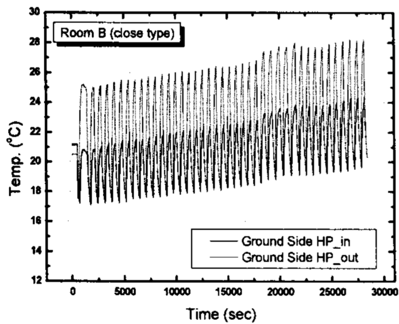
Fig. 7 Ground side water temperature variation of close type heat pumps
