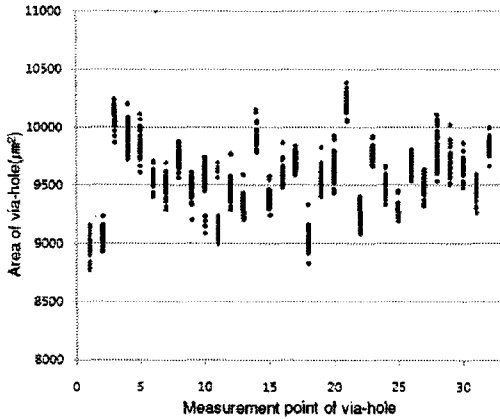
Fig. 9(a) Measurement of area
