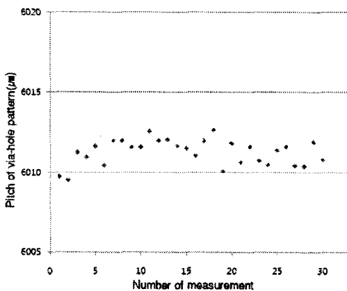
Fig. 9(c) Measurement of pitch
