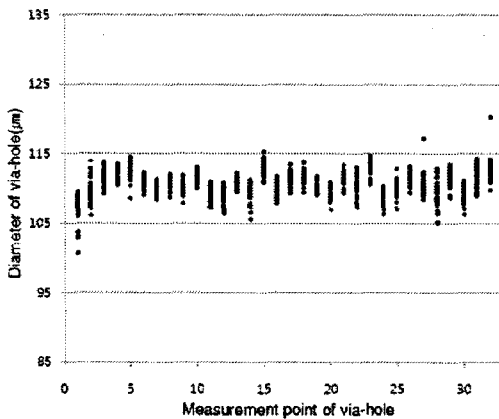
Fig. 9(b) Measurement of diameter
