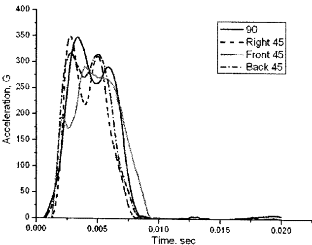
Fig. 2 HeadForm's acceleration vs time for impact sites in flat anvil
