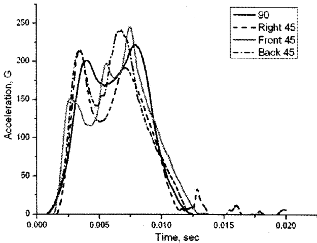
Fig. 3 HeadForm's acceleration vs time for impact sites in hemispherical anvil
