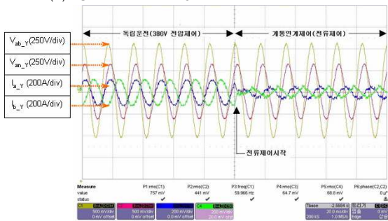
(c) 전압제어에서 전류제어모드로 전환 (c). Voltage control to Current control mode
