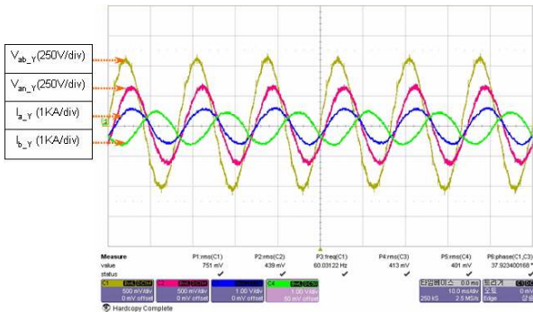
(d) 250kW 정격부하 운전(계통연계제어) (d) Rated power operation of 250kW PCS (Grid-connected)
