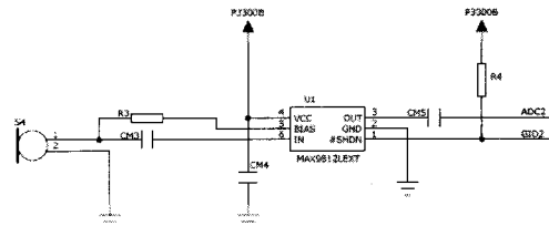
Microphone Sensor
